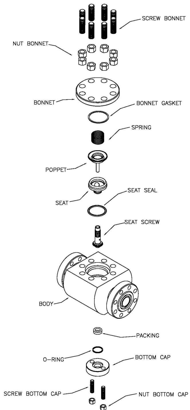
10,000 psi WP Check Valve
